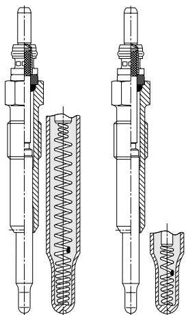
Inner structure of the self-controlling standard glow plug SR (left) and the performance-optimized glow plug of the ISS (right).
